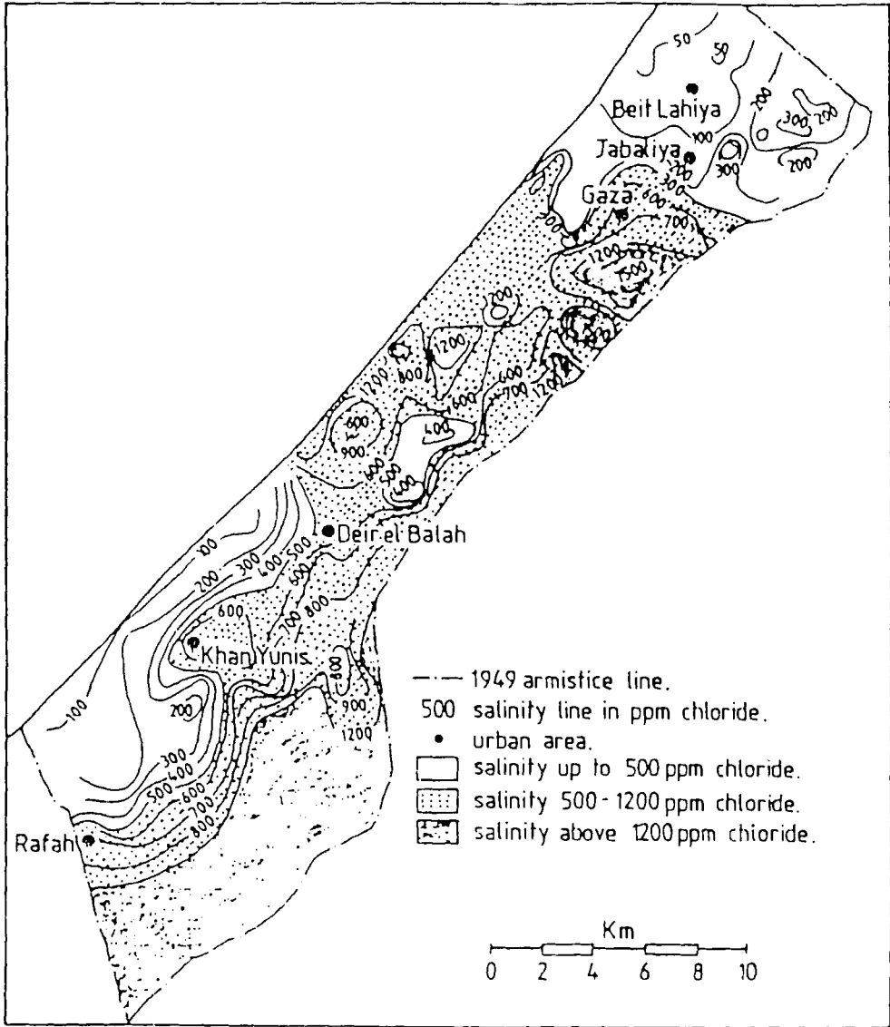
Figure 1: Salinity in the Gaza Strip, 1987-1988
