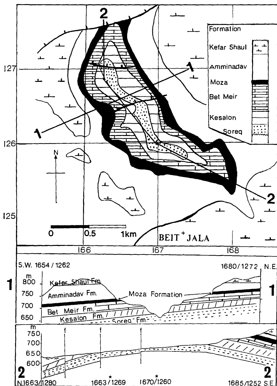
Fig. 5 The Wadi Ahmed (Cremisan Valley) geological map and sections (a) Geological section across Wadi Ahmed (1); (b) Geological section along axis of Wadi Ahmed (2).
