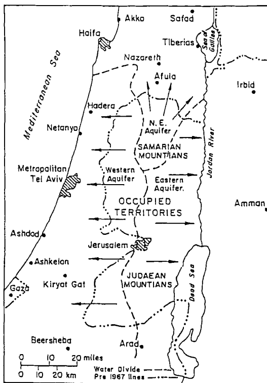
Figure 1. The Mountain Aquifer-A Schematic Presentation: The pre-1967 cease fire line which serves as the border between Israel and the occupied territories (West Bank), mainly inhabited by the Palestinians, is shown with a heavy dashed and dotted line. The hydrological divide between the three subdivisions within the mountain aquifer is shown by the dashed line. The arrows show the general direction of the flow of the ground water.
