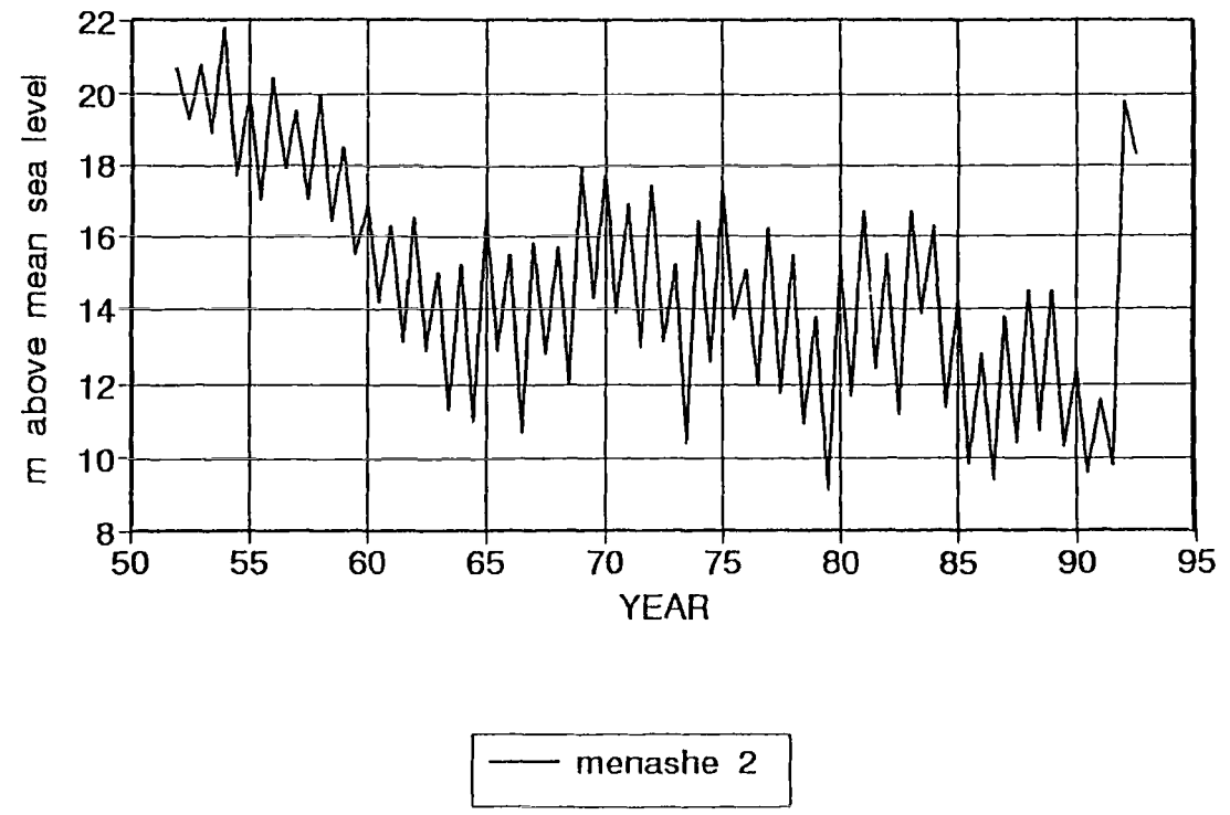
Fig. 5 Water Level in the Yarqon Tanninin Aquifer
